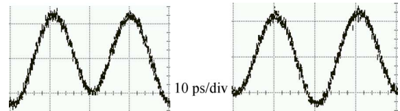
Fig. 1. Received intensity modulation (64-fold averaged) for the two polarization channels (while clock recovery PLL stays locked).
