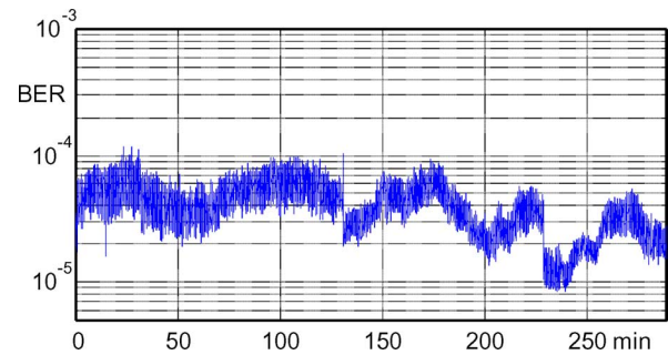
Fig. 7. BER performance while transmitting over 430 km during almost 5 h with 40-krad/s polarization scrambling rate.
